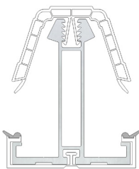
Rafter
